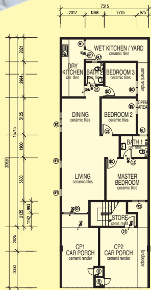
Lower Ground 2 - Type A1
