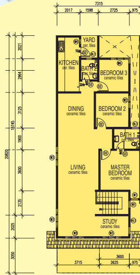
Lower Ground 1 - Type A2
