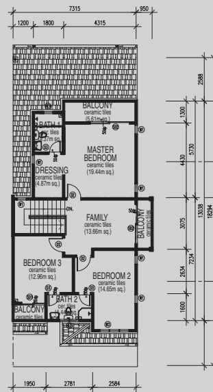
Second Floor - Type B2
