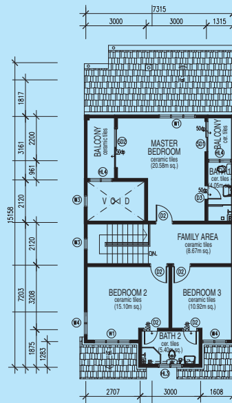
First Floor - Type D3
