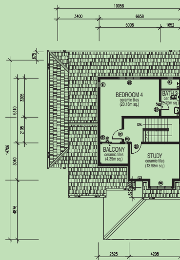
Second Floor - Type C2
