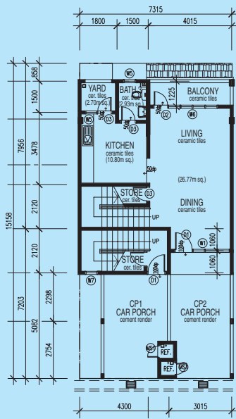
Ground Floor - Type D2
