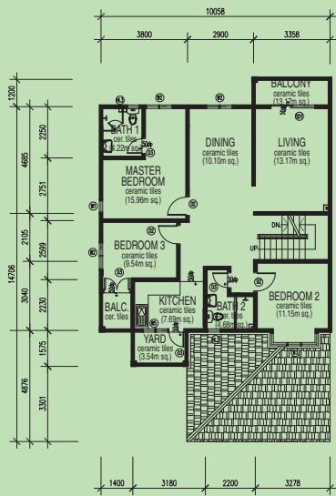
First Floor - Type C2
