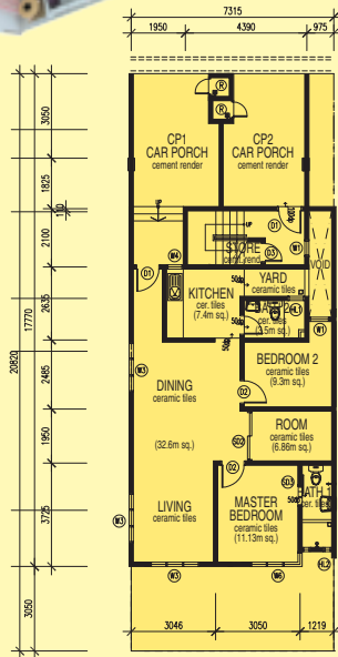
Ground Floor - Type A3
