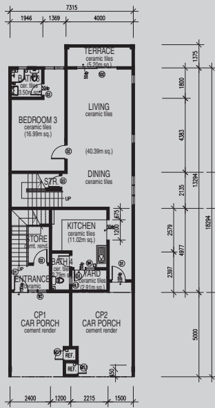
Ground Floor - Type B1
